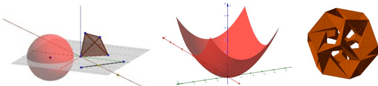
Figure 8: GeoGebra3D
